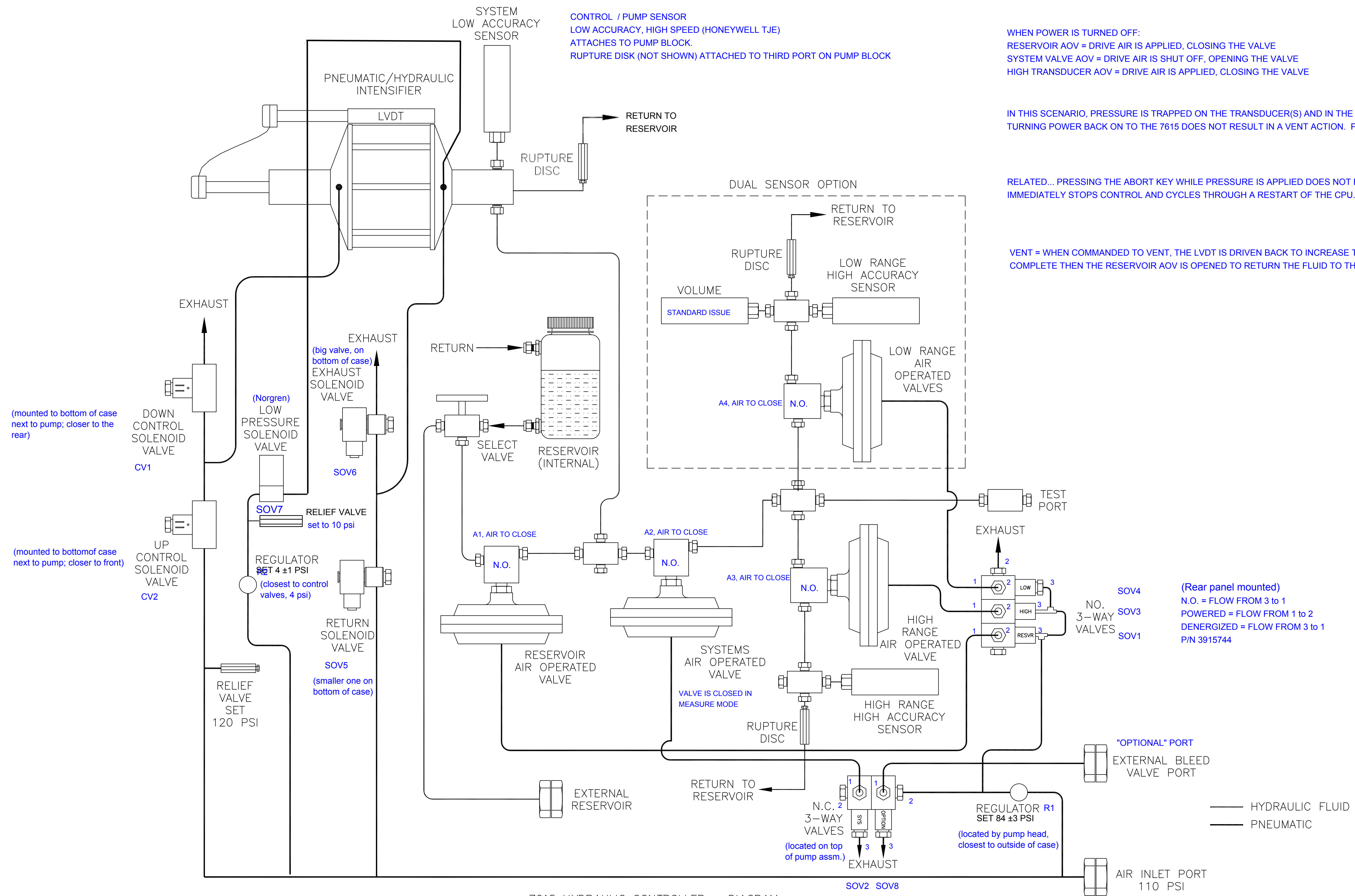
7615 HYDRAULIC CONTROLLER - DIAGRAM
